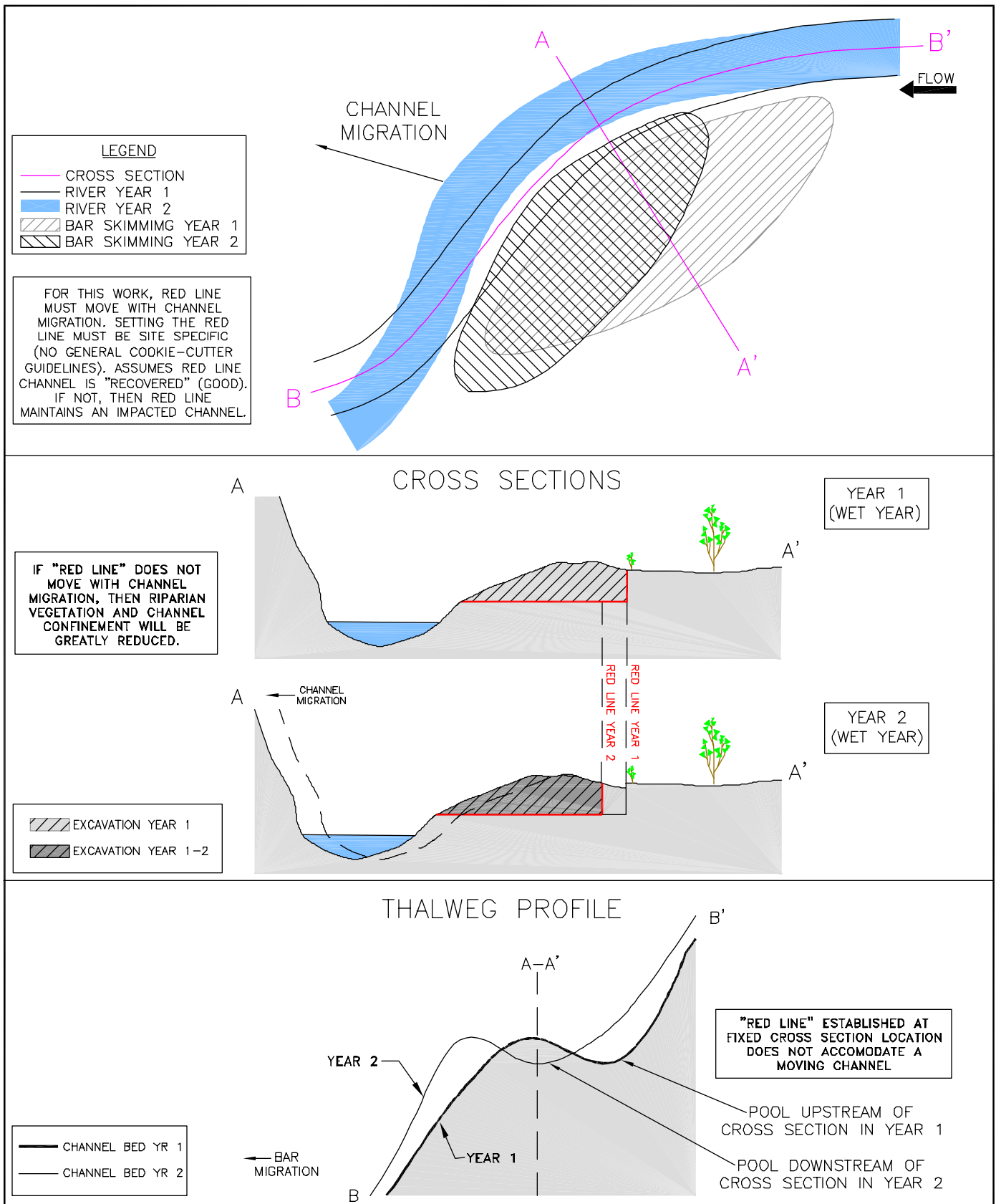
FIGURE 7. ANNUAL REPLENISHMENT (RED LINE) STRATEGY
