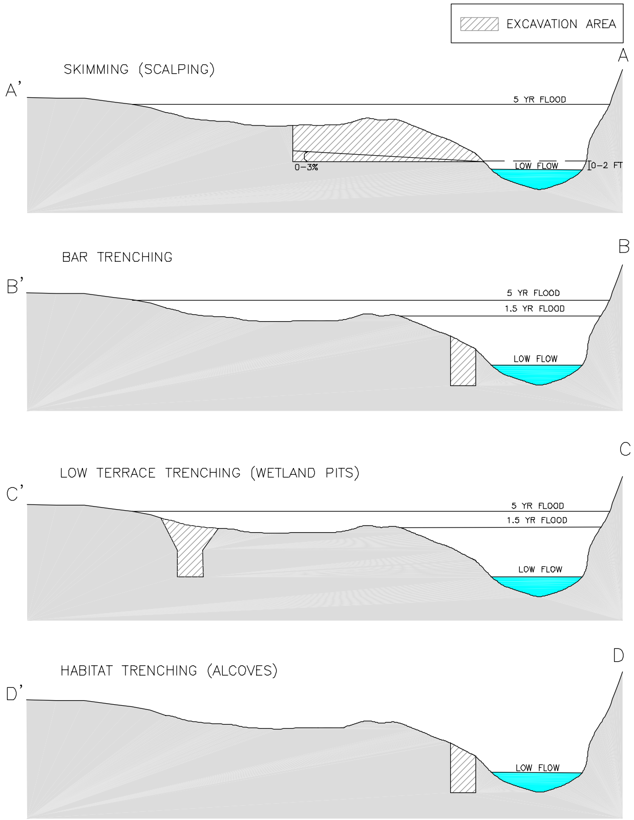
FIGURE 10. DIAGRAMS OF CONTEMPORARY GRAVEL EXCAVATION METHODS (SEE FIGURE 5 FOR PLANVIEW)
