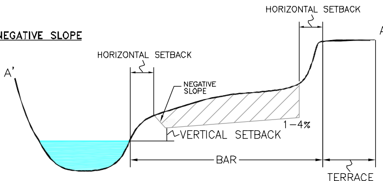
FIGURE 3. TYPICAL SETBACK STANDARDS
