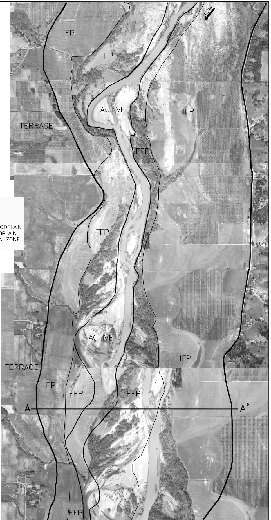
FIGURE 8. 1940 AIRPHOTO OF AN ALLUVIAL RIVER SHOWING LATERAL ZONES WITHIN THE RIVER CORRIDOR
